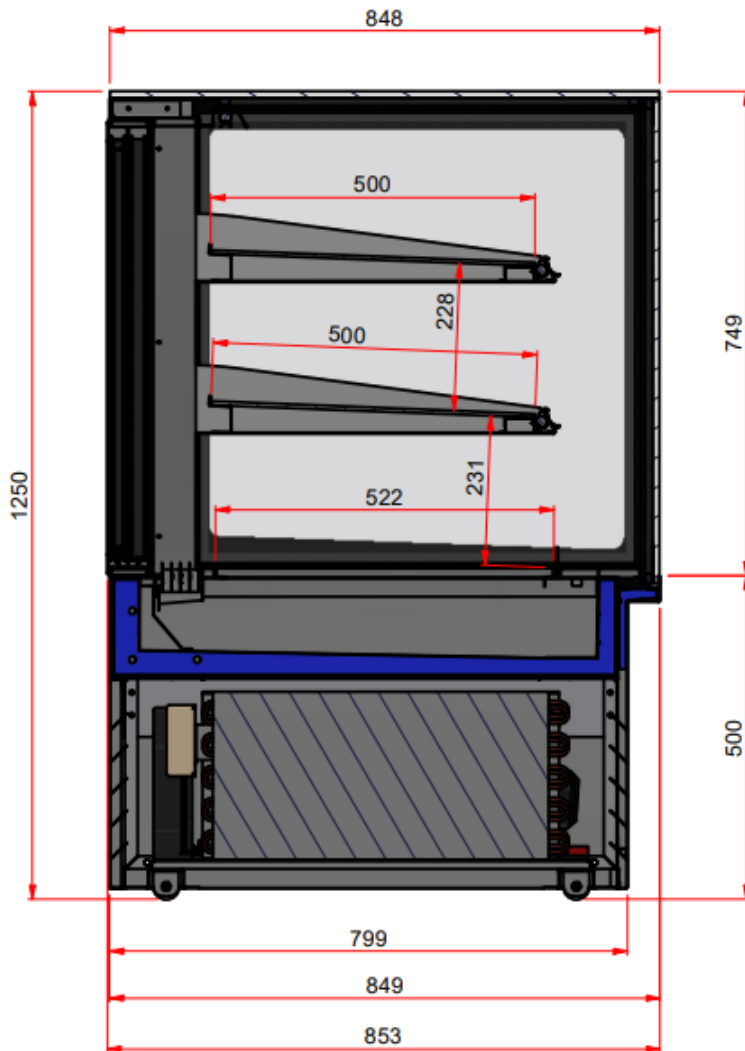
SIDE SECTION VIEW
